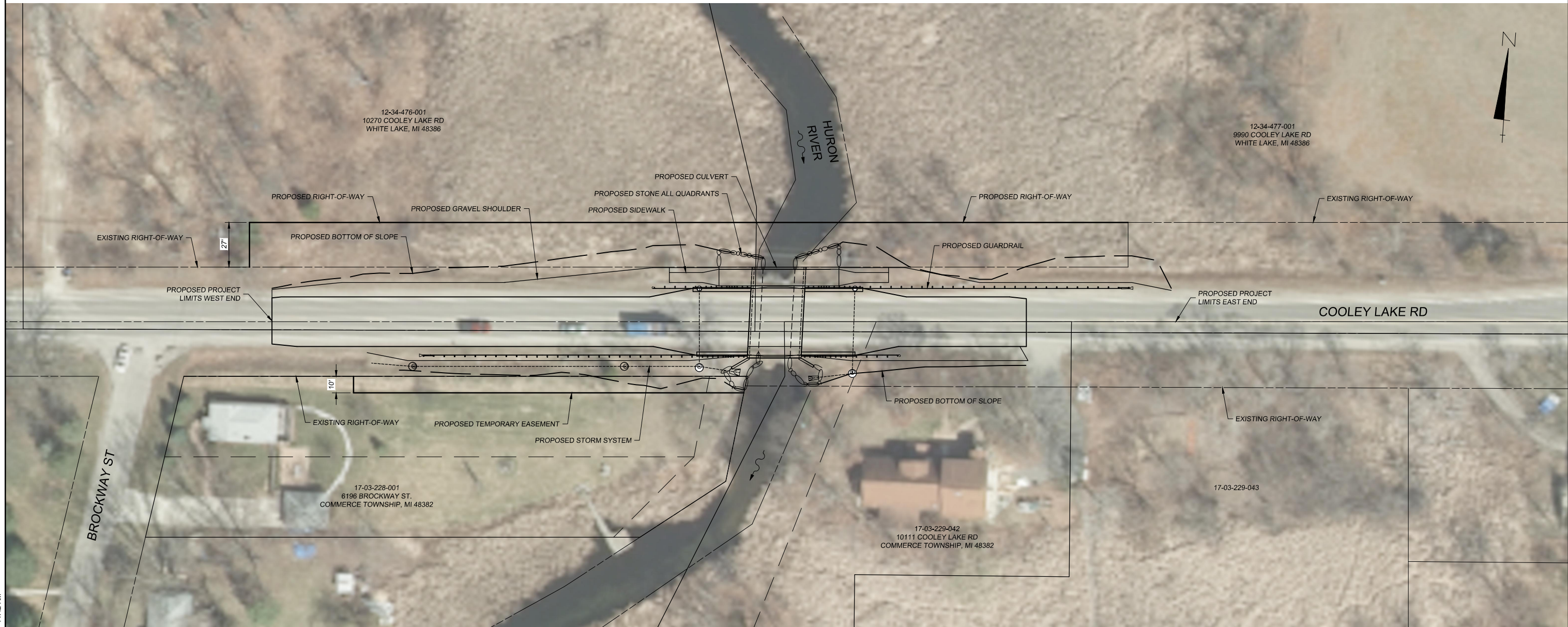
SITUATION PLAN
